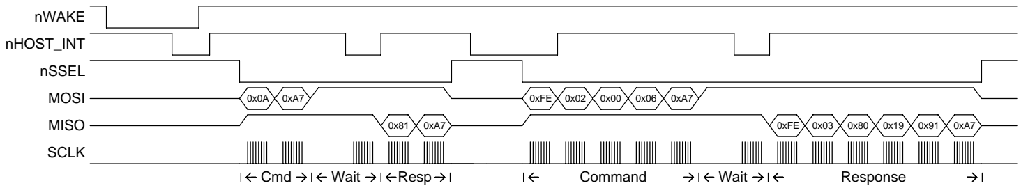
Figure 11. Timing Diagram of the Three-Part Transaction
