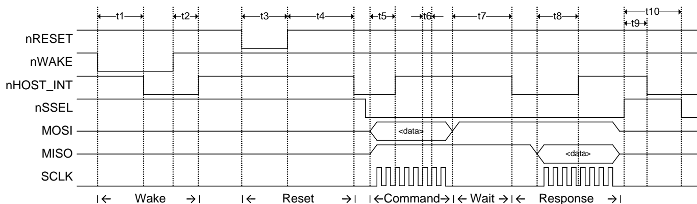
Figure 6. SPI Protocol Timing Waveform
