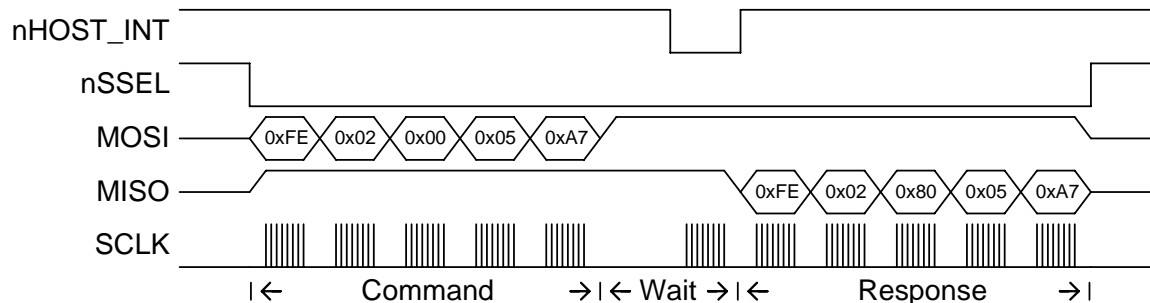
Figure 9. EmberZNet Serial Protocol Frame - NOP Command Example
