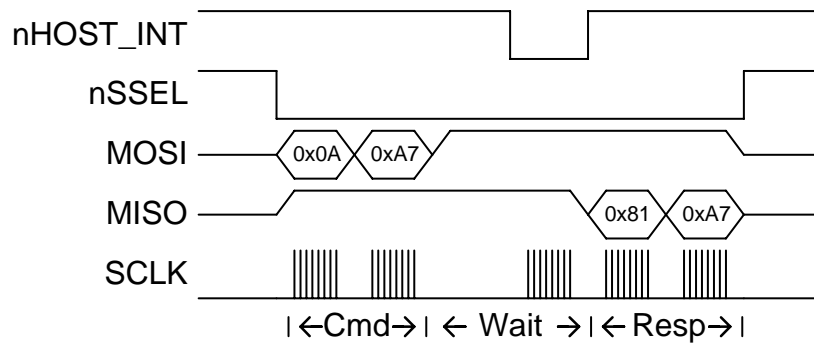
Figure 8. SPI Protocol Version Example
