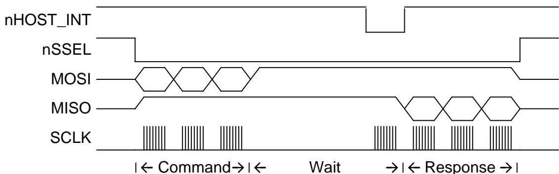
Figure 4. General Timing Diagram for a SPI Transaction
