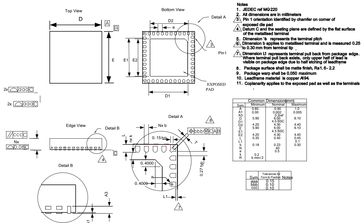
Figure 13. Package Drawing
