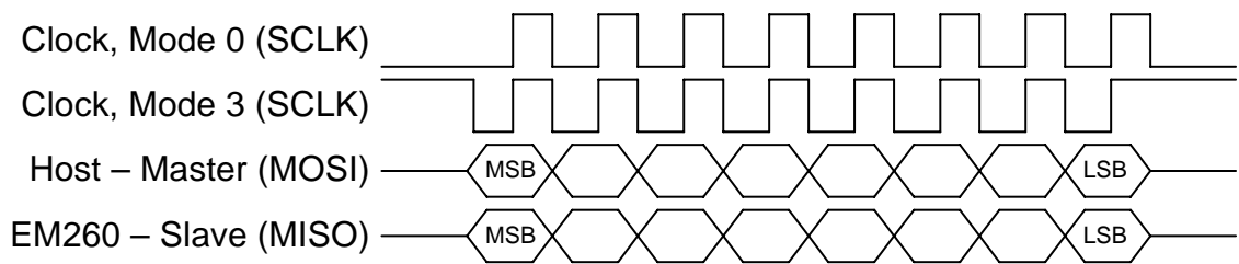
Figure 3. SPI Transfer Format, Mode 0 and Mode 3
