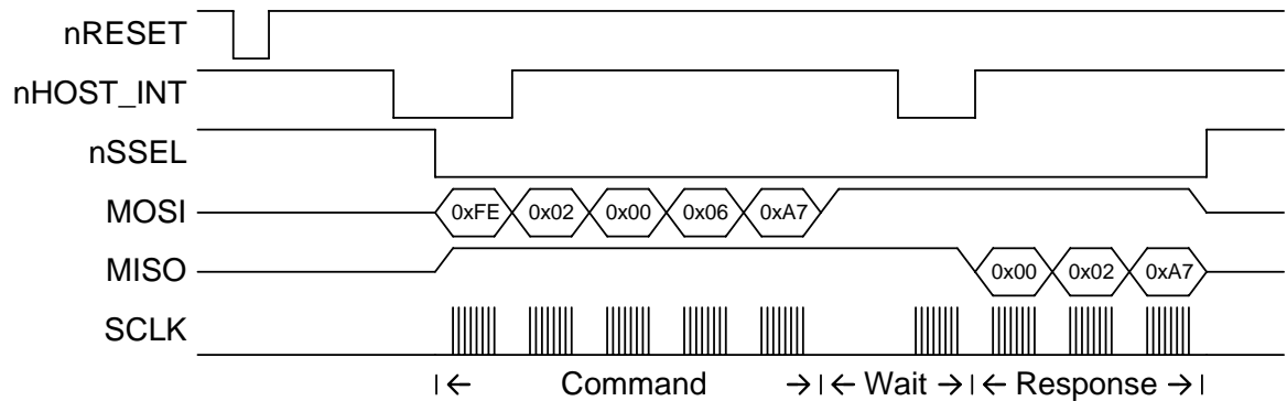
Figure 10. EM260 Reset Example
