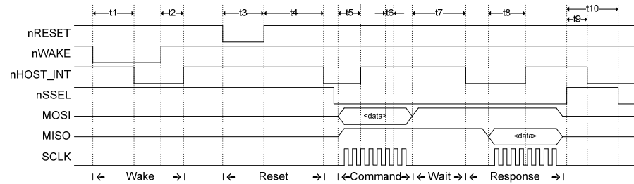
Figure 4. SPI Protocol Timing Waveform
