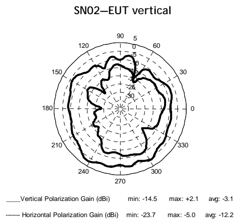
Figure 9. Measured antenna patterns for EM250 62 mil boards
